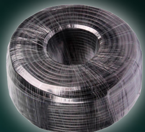
LWR6 6 Core Wire 2*1 mm 2 Power Cable + 4*0.3 mm 2 Signal Wire 250 feet or 500 feet / roll
