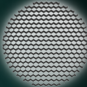
HC02 Honeycomb Filter For PAR36 Fixtures Black 4.3" (L) x .1" (W)
