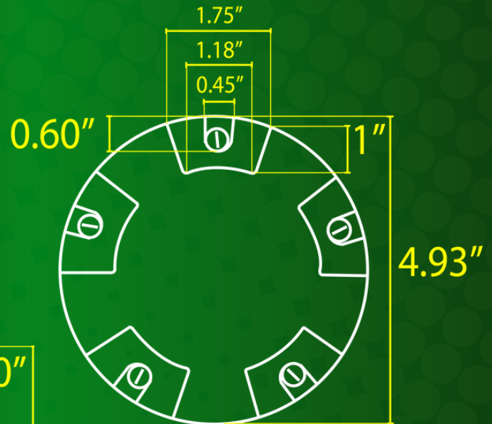
TOP FIXTURE ANGLE
